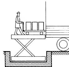
8 Dock to truck
